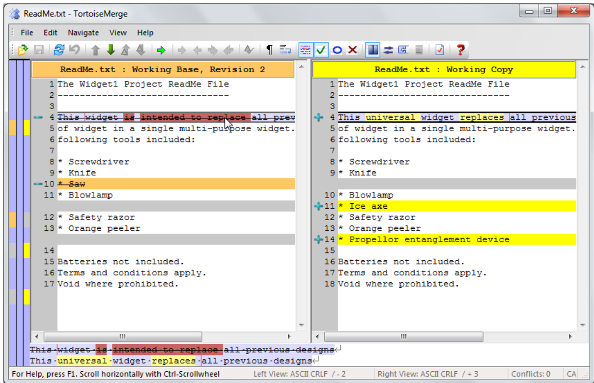
Slika 1.3. File Difference Viewer
