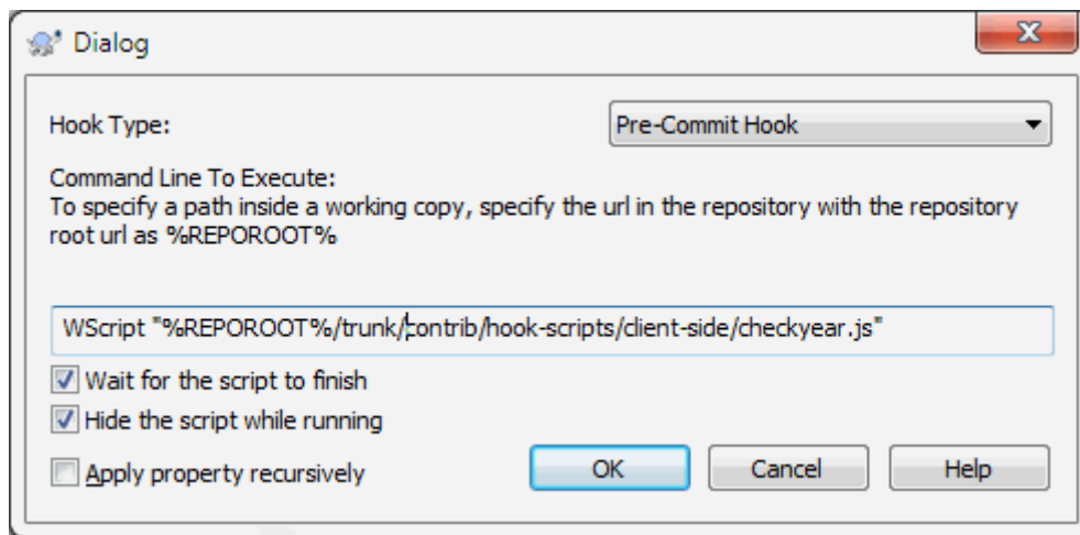
Slika 4.36. Property dialog for hook scripts
