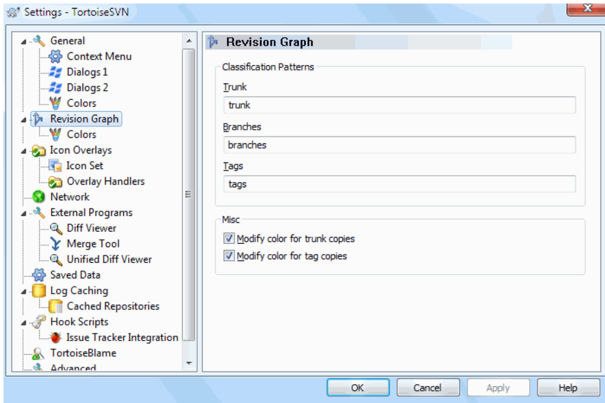
Slika 4.74. The Settings Dialog, Revision Graph Page
